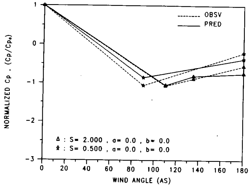
FIGURE 2-8 NORMALIZED PRESS. COEFF. VS WIND ANGLE
