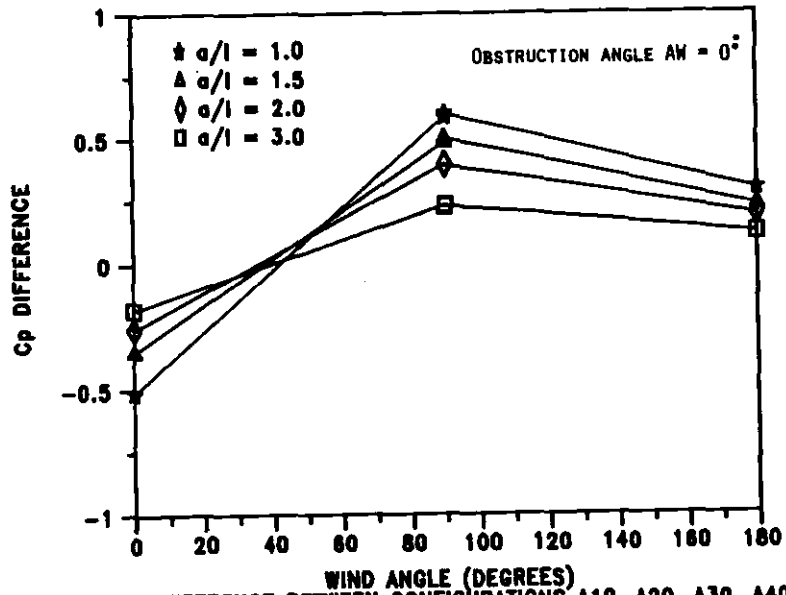
FIG. 2-52: C_p DIFFERENCE BETWEEN CONFIGURATIONS A10, A20, A30, A40 AND UNOBSTRUCTED BUILDING CONFIGURATION (A00).
