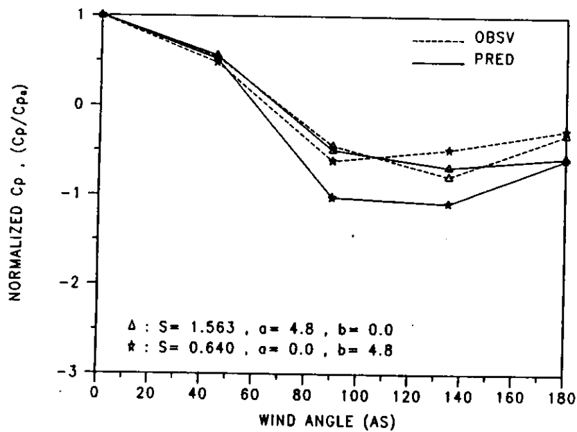
FIGURE 2-19 NORMALIZED PRESS. COEFF. VS WIND ANGLE
