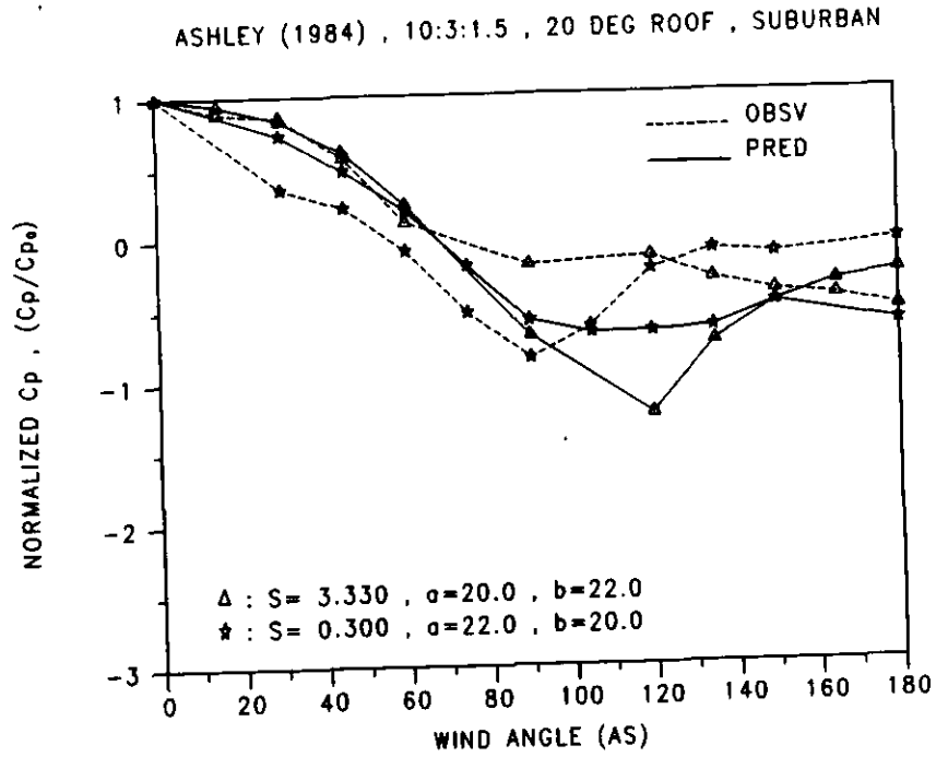
FIGURE 2-30 NORMALIZED PRESS. COEFF. VS WIND ANGLE
