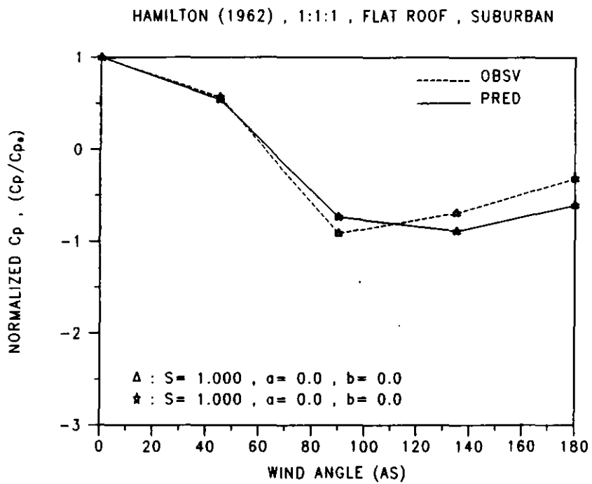
FIGURE 2-13 NORMALIZED PRESS. COEFF. VS WIND ANGLE
