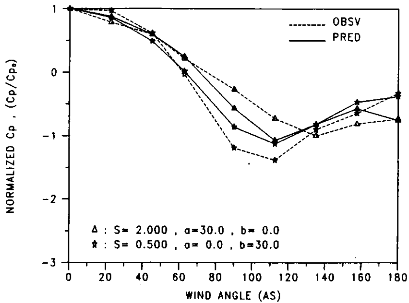
FIGURE 2-26 NORMALIZED PRESS. COEFF. VS WIND ANGLE
