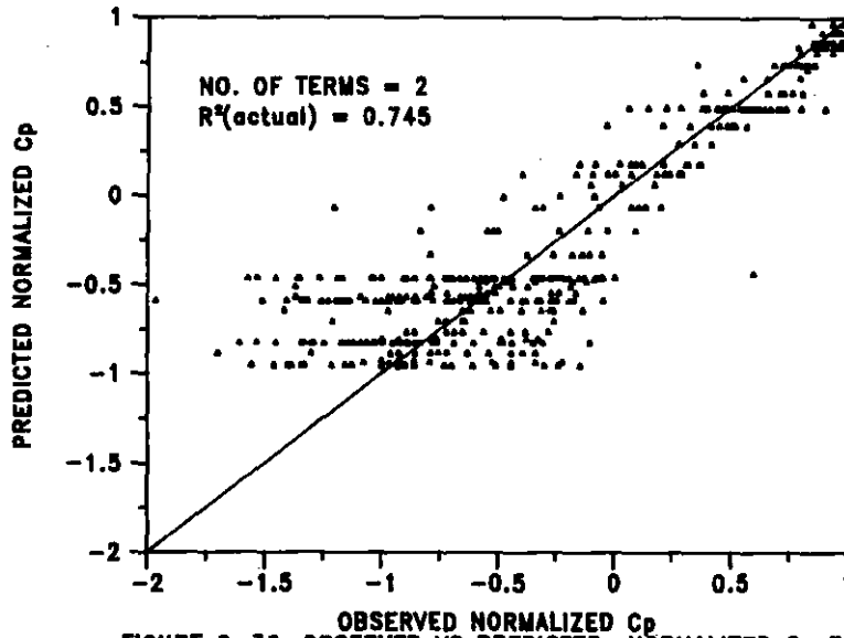
FIGURE 2-36: OBSERVED VS PREDICTED NORMALIZED C_p FOR DIFFERENT NUMBER OF TERMS IN THE PREDICTION EQUATION
