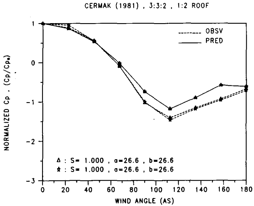
FIGURE 2-12 NORMALIZED PRESS. COEFF. VS WIND ANGLE
