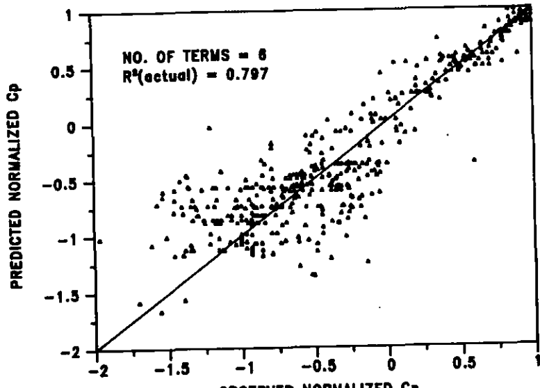
FIGURE 2-40: OBSERVED VS PREDICTED NORMALIZED Cp FOR DIFFERENT NUMBER OF TERMS IN THE PREDICTION EQUATION
