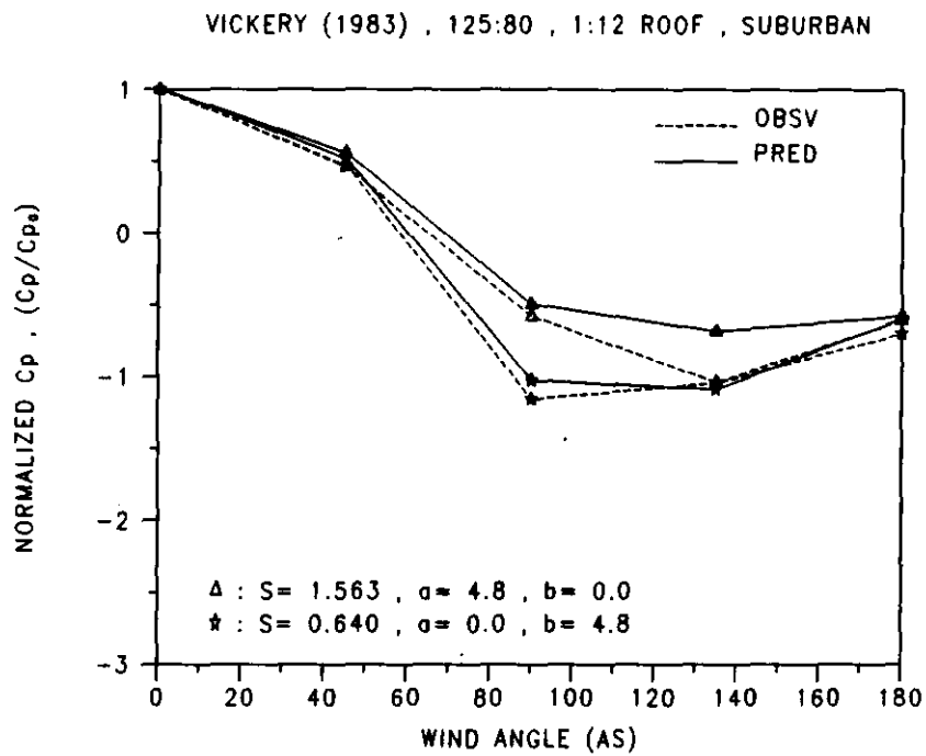
FIGURE 2-21 NORMALIZED PRESS. COEFF. VS WIND ANGLE
