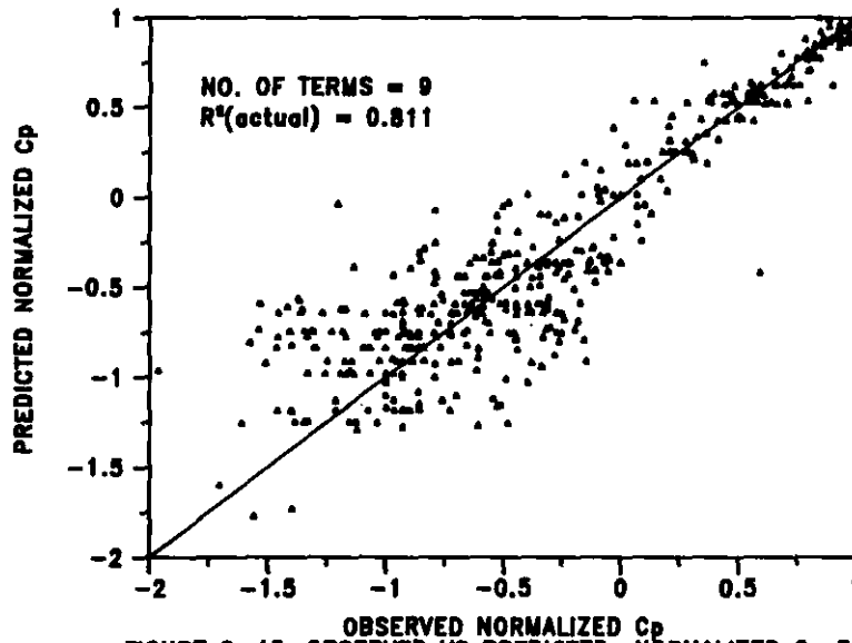
FIGURE 2-43: OBSERVED VS PREDICTED NORMALIZED Cp FOR DIFFERENT NUMBER OF TERMS IN THE PREDICTION EQUATION
