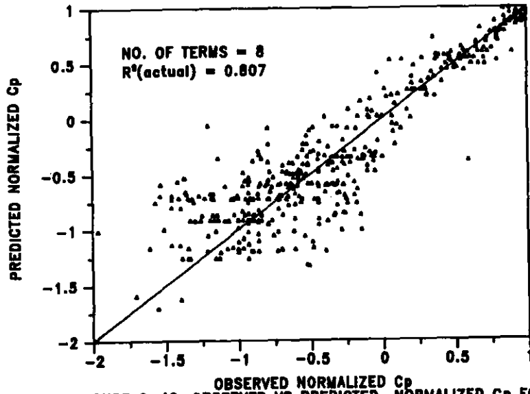
FIGURE 2-42: OBSERVED VS PREDICTED NORMALIZED Cp FOR DIFFERENT NUMBER OF TERMS IN THE PREDICTION EQUATION
