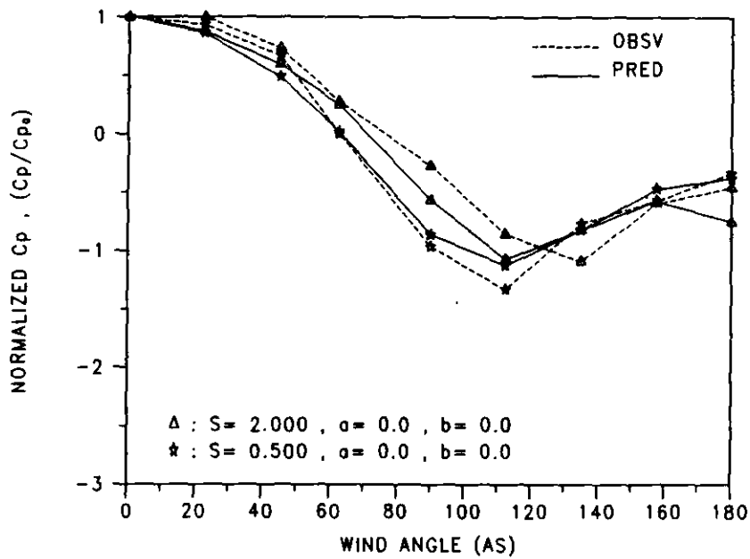
FIGURE 2-23 NORMALIZED PRESS. COEFF. VS WIND ANGLE
