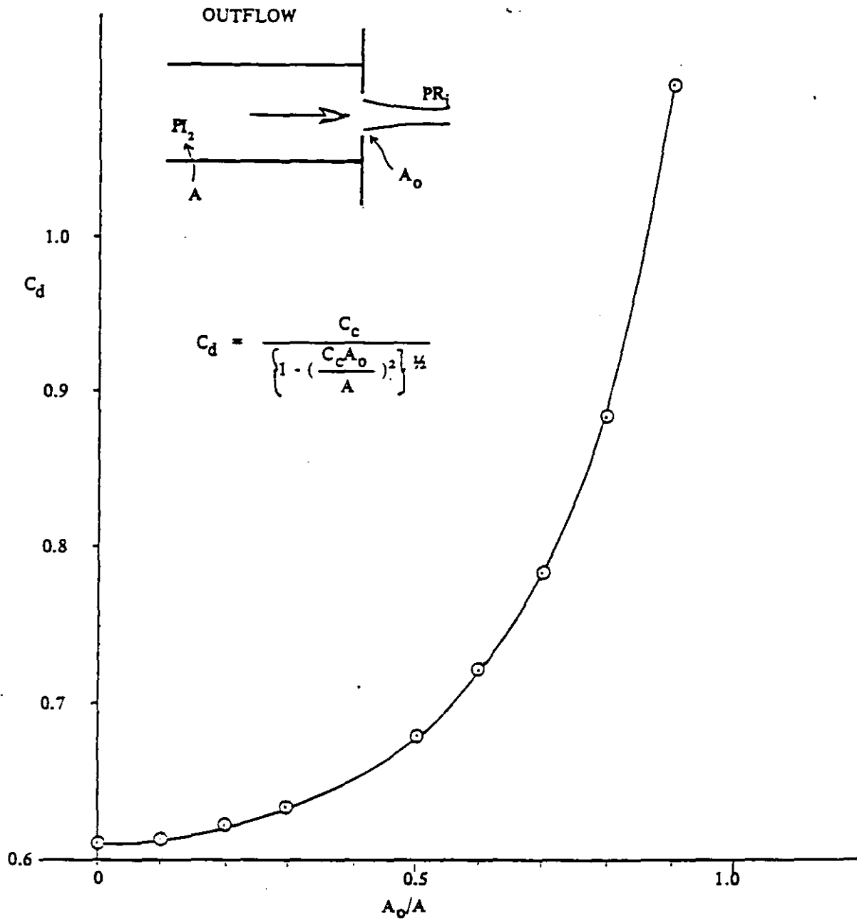
Figure 2-62 DISCHARGE COEFFICIENTS FOR HIGH REYNOLD NUMBER FLOWS (From VICKERY)
