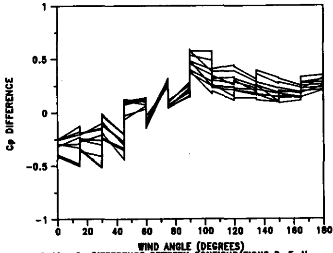
FIG. 2-46: C_p DIFFERENCE BETWEEN CONFIGURATIONS D, F, H AND UNOBSTRUCTED BUILDING CONFIGURATION (A00).
