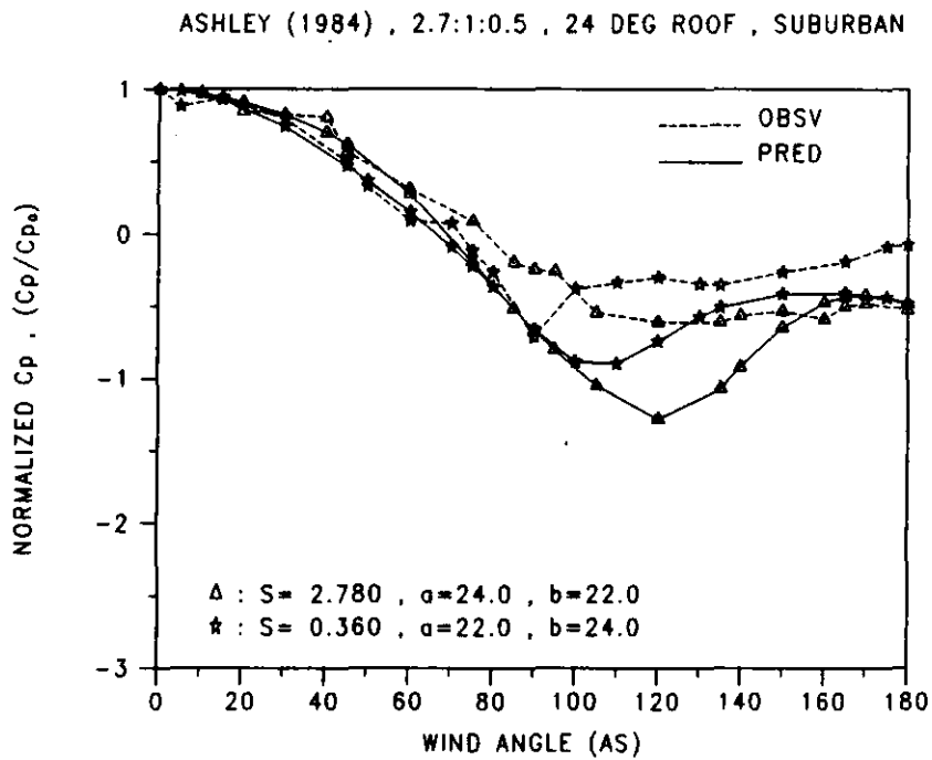
FIGURE 2-31 NORMALIZED PRESS. COEFF. VS WIND ANGLE
