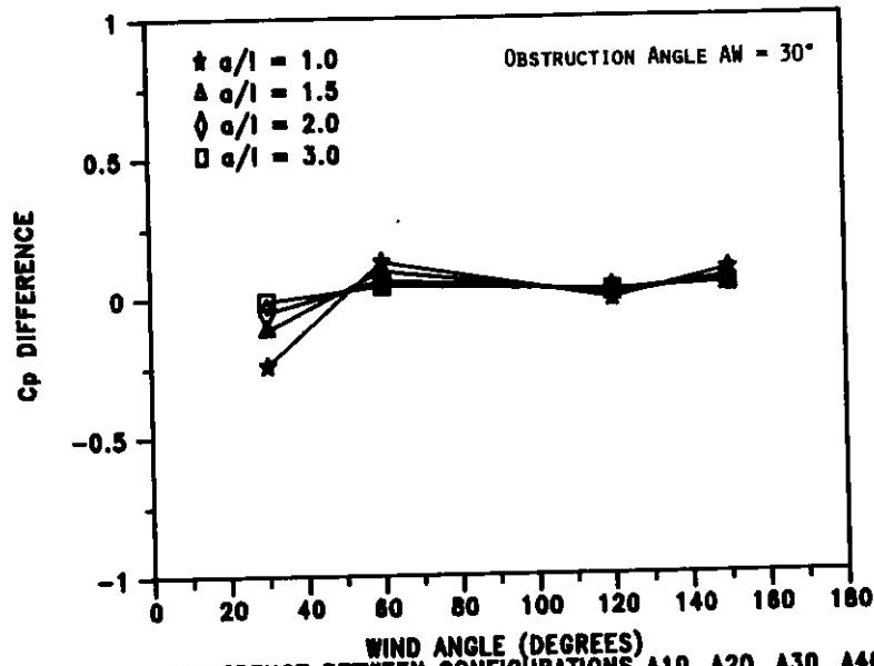
FIG. 2-54: C_p DIFFERENCE BETWEEN CONFIGURATIONS A10, A20, A30, A40 AND UNOBSTRUCTED BUILDING CONFIGURATION (A00).
