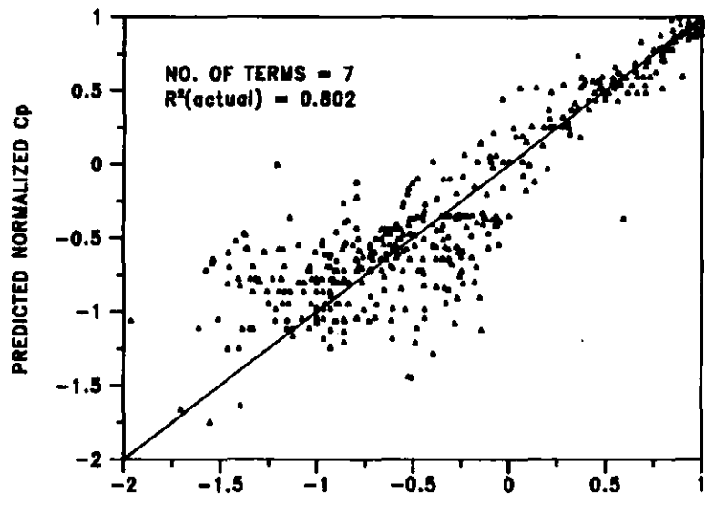
FIGURE 2-41: OBSERVED VS PREDICTED NORMALIZED Cp FOR DIFFERENT NUMBER OF TERMS IN THE PREDICTION EQUATION
