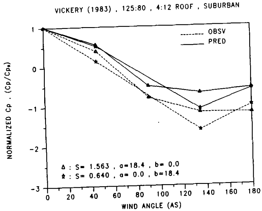
FIGURE 2-20 NORMALIZED PRESS. COEFF. VS WIND ANGLE
