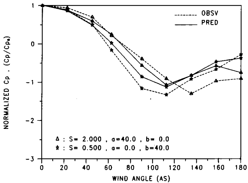
FIGURE 2-27 NORMALIZED PRESS. COEFF. VS WIND ANGLE
