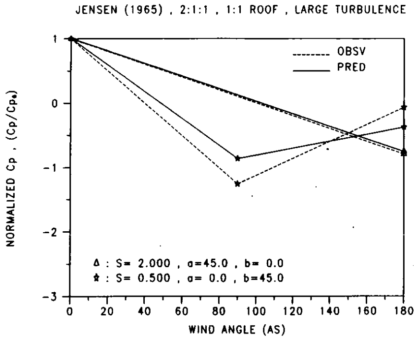
FIGURE 2-10 NORMALIZED PRESS. COEFF. VS WIND ANGLE
