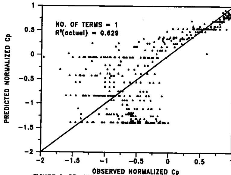
FIGURE 2-35: OBSERVED VS PREDICTED NORMALIZED C_p FOR DIFFERENT NUMBER OF TERMS IN THE PREDICTION EQUATION
