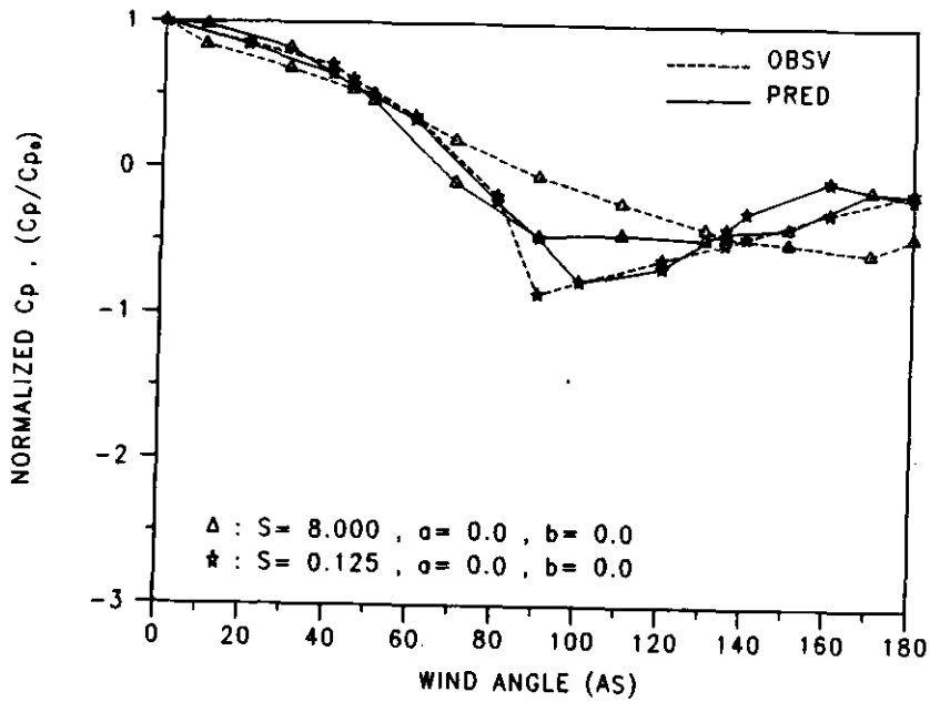
FIGURE 2-29 NORMALIZED PRESS. COEFF. VS WIND ANGLE
