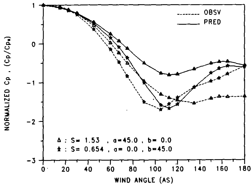
FIGURE 2-22 NORMALIZED PRESS. COEFF. VS WIND ANGLE
