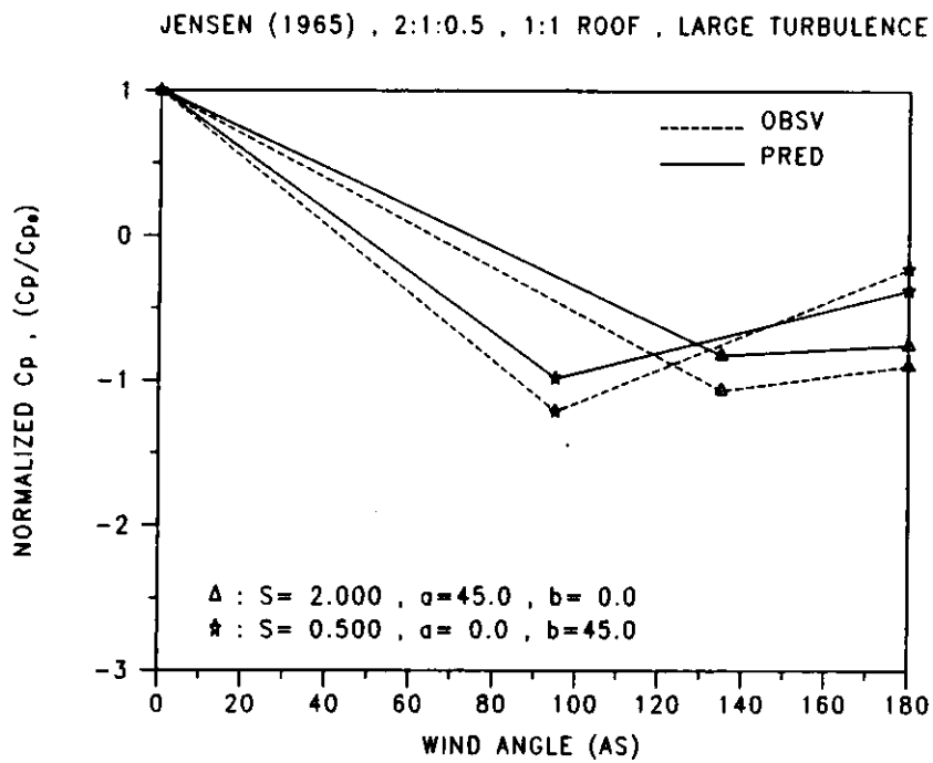
FIGURE 2-11 NORMALIZED PRESS. COEFF. VS WIND ANGLE
