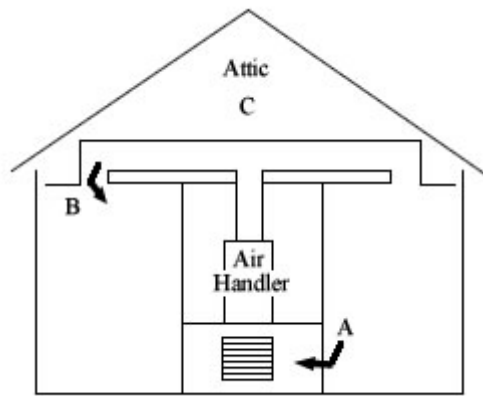
Figure 1. Procedure for determining proportion of return air coming from attic. Measure SF6 concentration at near return air grill, (B) at supply and (C) in attic.
