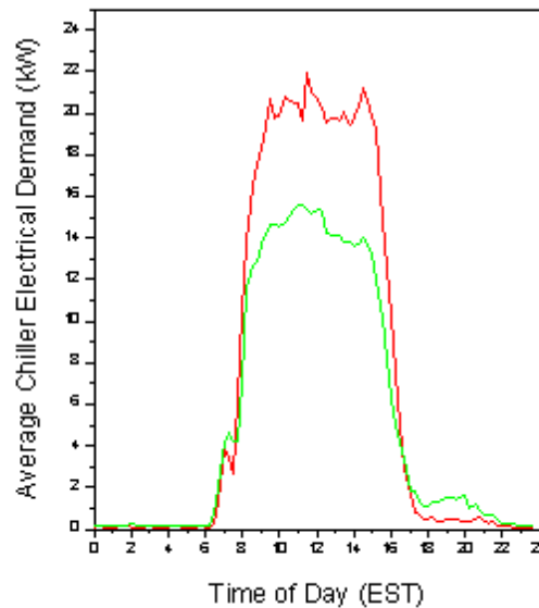
Chiller Summer Demand Profile: Weekdays, Pre (June - Sept. '94) and Post Roof Resurfacing (June - Sept '95)
