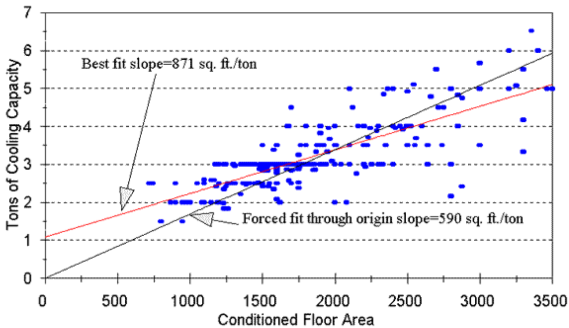
Figure 3. Regression of Cooling Capacity on Floor Area for Most Recent New Home AC Installation
