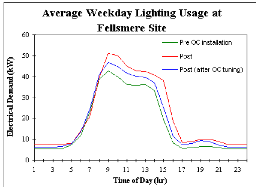
Figure 5. Fellsmere Elementary Before and After the OC Installation
