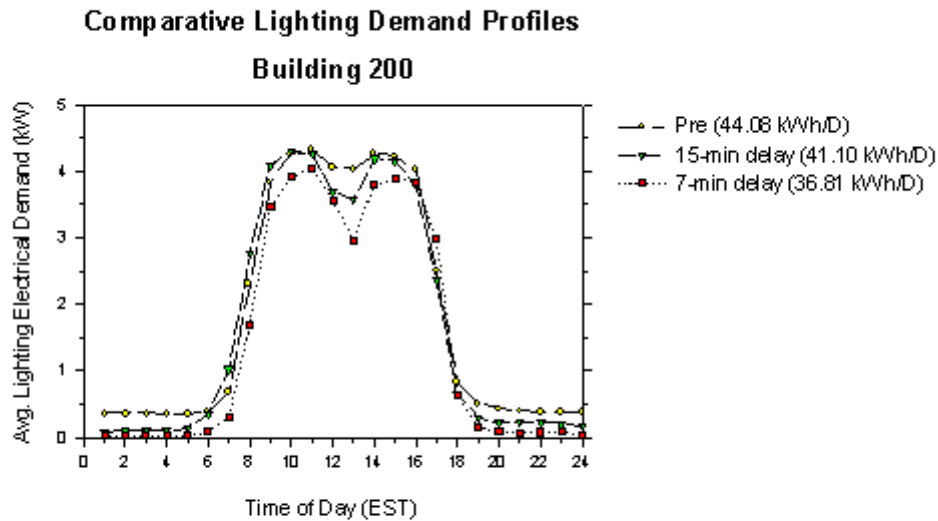
Figure 2. Building 200 Pre and Post Period Load Profiles
