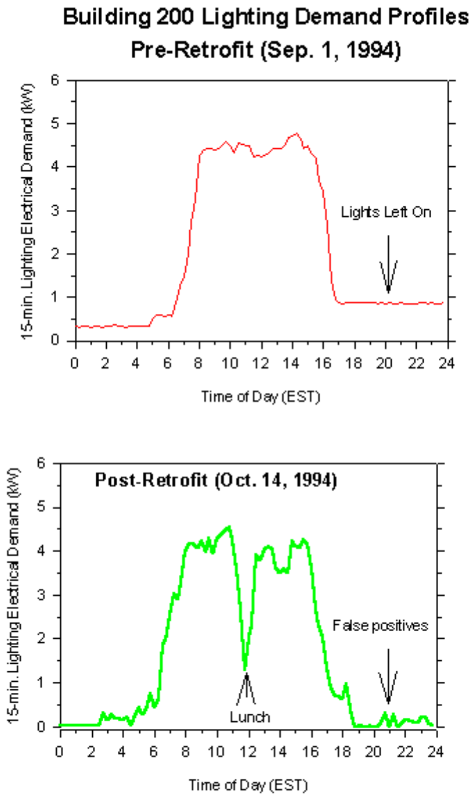
Figure 1. Sample Daily Load Profiles for Building 200
