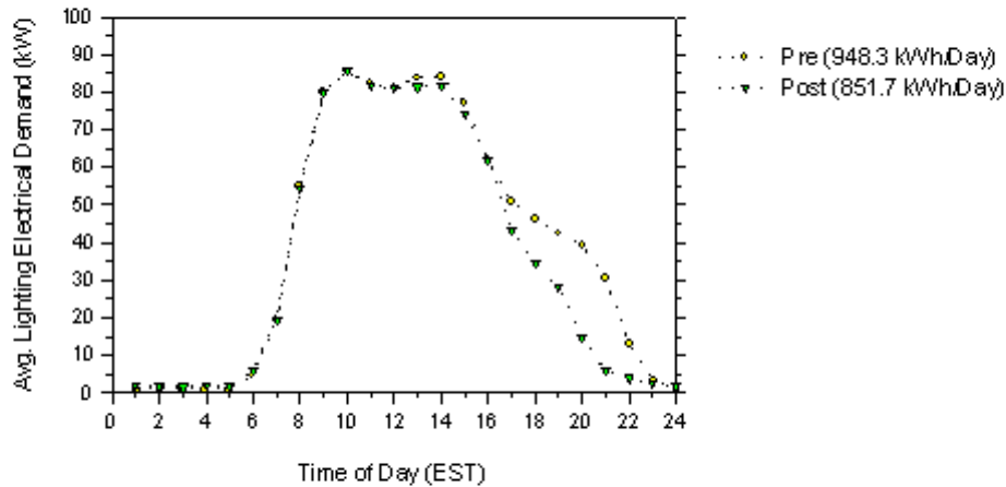
Figure 3. Northwest Elementary Lighting Load Shapes Before and After the OC Installation
